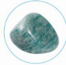
Amazonite
